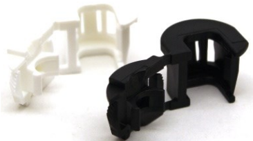
126 WHT/BK Lock-It Style Strain Relief for .875" PF Hole for 12/3, 14/3, 14/4 & 18/5 .380"-.450" cord
