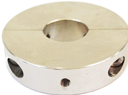
Stabilizer Ring 3/8" IP 2" OD x .5"H 3-Tapped 8/32" Holes For Gripper Studs M-4 Screws to Clamp
