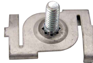
#138 1/4"-20 Stud on a Twist Clip for Acoustical T-Bar
