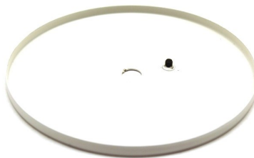
#93B Stud Canopy 5" Diameter x .25" H .400" Center Hole 8/32" Stud with Lock Washer Available in White, Black, Brushed Nickel or Nickel Also available 5" Square Canopy - White, Black, Brushed Nickel, or Nickel
