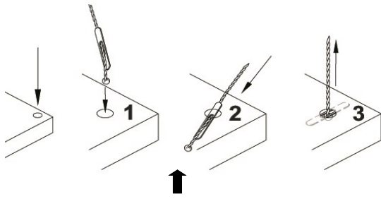
Paddle insertion into fixture
