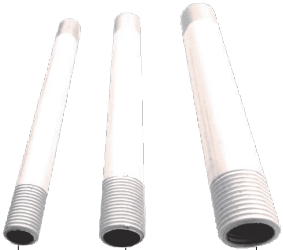
1/4"IPS .500"-.510"O.D. 18 T.P.I. 3/8"IPS .625"-.635"O.D. 18 T.P.I. 1/2"IPS .800"-.810" O.D. 14 T.P.I. T.P.I.=Threads Per Inch I.P.S.=Iron Pipe Standard
